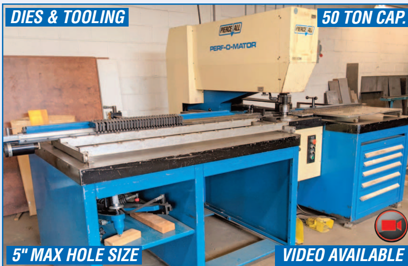
PIERCE-ALL 3050 PERF-O-MATOR SINGLE STATION TURRET PUNCH
